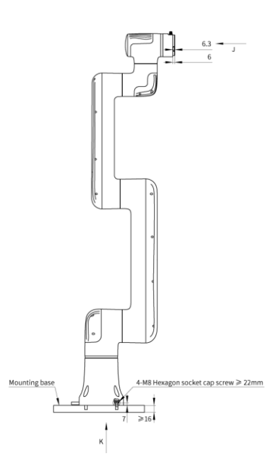
▲ Mounting hole diagram
