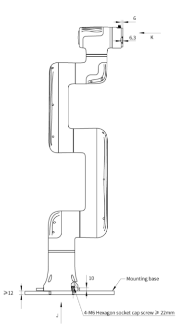
▲ Mounting hole diagram
